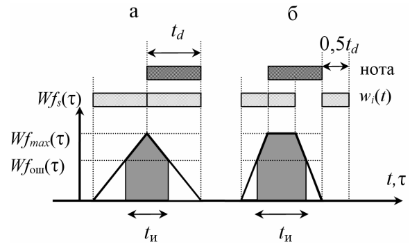
Fig. 8. Envelopes of correlation function of note and wavelet w(t) corresponding to the frequency of scale note pitch
