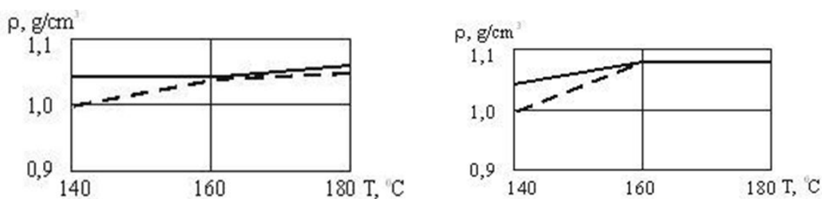
Figure 2. Dependence of amber density on the distortion temperature: heating time – 1 h (a), 2 h (b)
