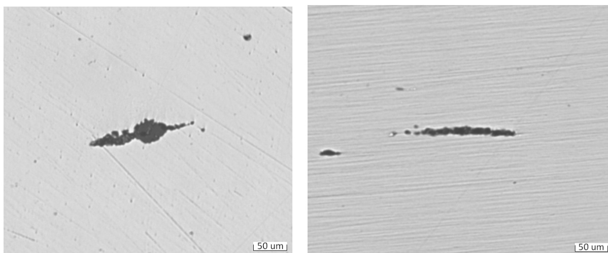
Figure 1. Kind of typical non-metallic inclusions, occurring in the metal products 2A82-1M
