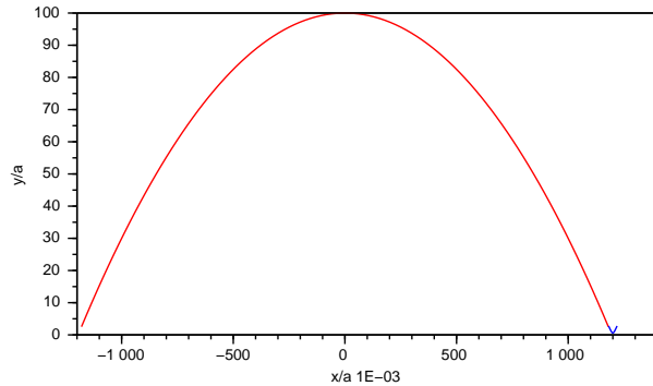
Figure 3. One period of trajectory of a charged particle. H = 50 kOe, mc^2 = 40 MeV, eU_0 = 30 eV, a = 1 Å, \varepsilon = 0.5 .
