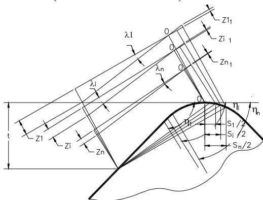
Fig. 5: Scheme to the determination of coordinates of chip formation surface for the condition of constant cutting depth
