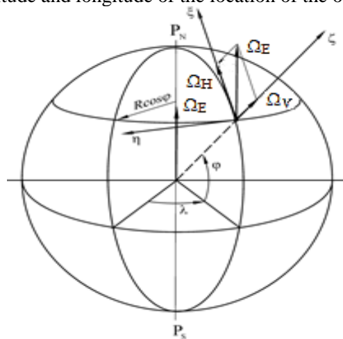
Figure 1. Geographically oriented earth axis system.
