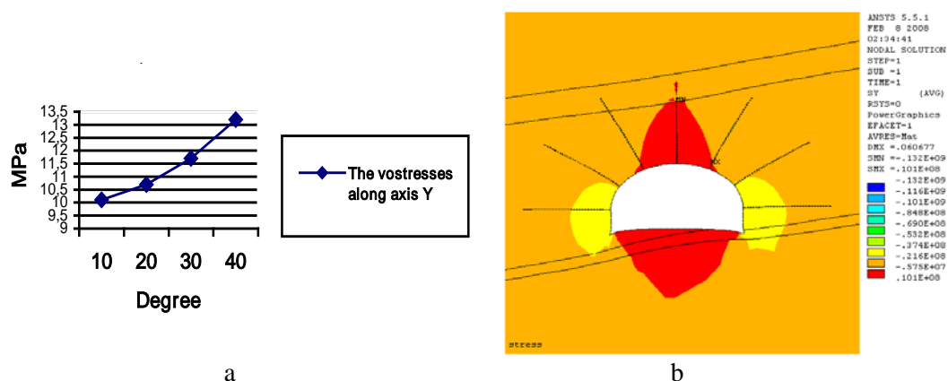
Figure 4. The change and distribution of the maximum stresses in the zones surrounding mine working.
