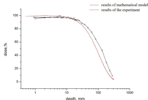
b) the distribution of the absorbed dose in the depth of the phantom
