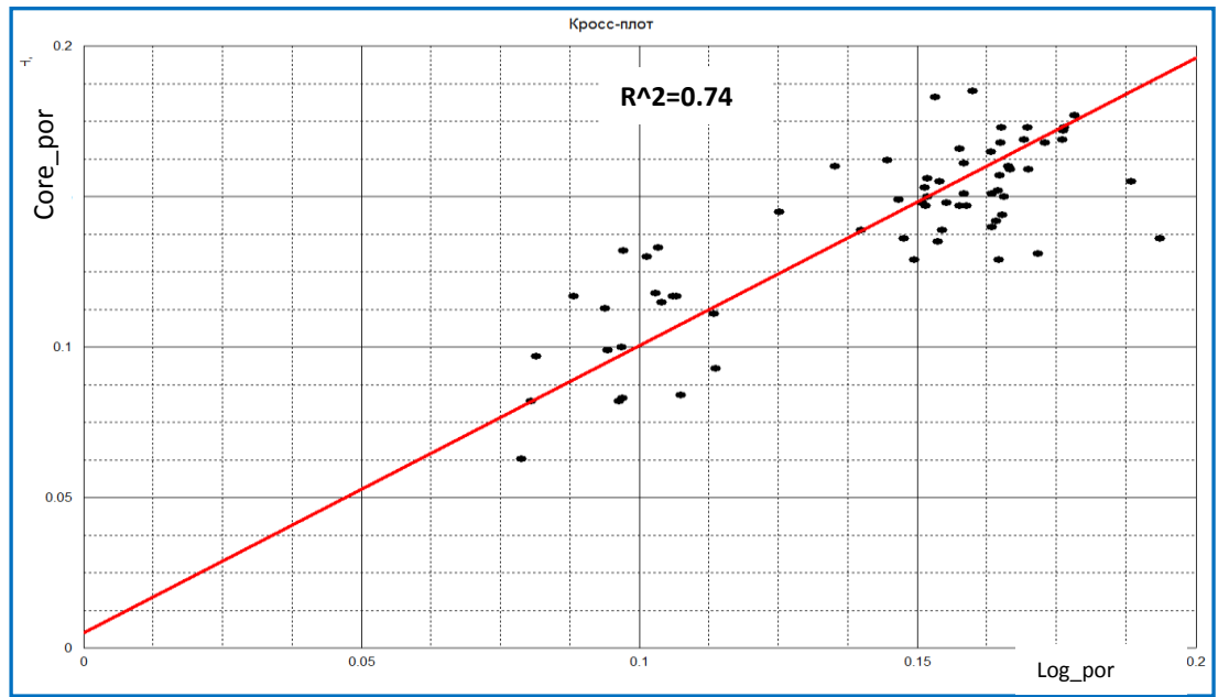
Figure 3.8 Correlation of Acoustic effective porosity (SP) vs Core porosity
