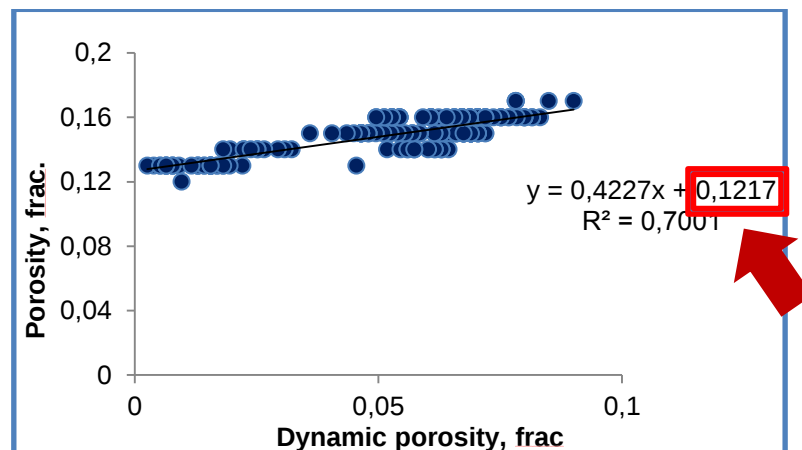
Figure 3.23 Porosity critic value determination
