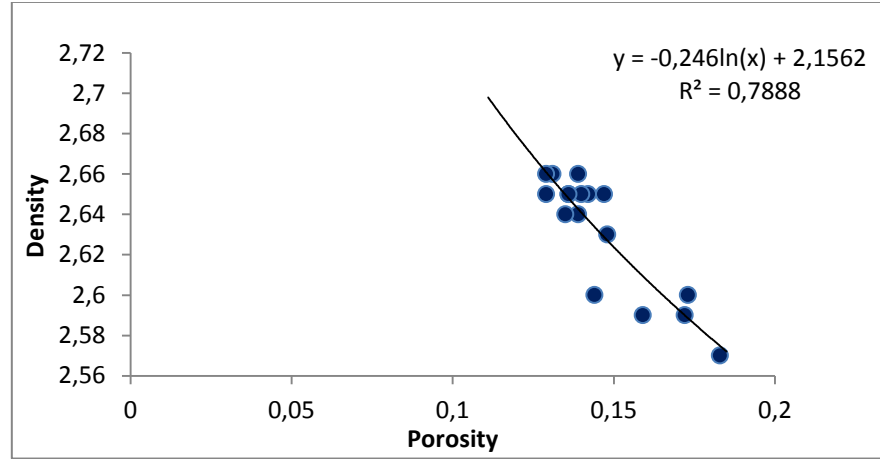
Figure 3.9 Core density and porosity relationship
