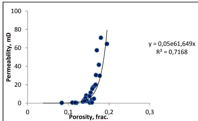
Fig. 3.11 Core permeability and porosity relationship
