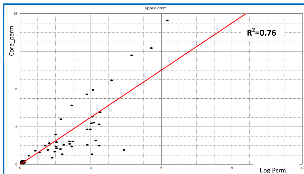
Figure 3.12 Correlation of base permeability value vs core permeability data
