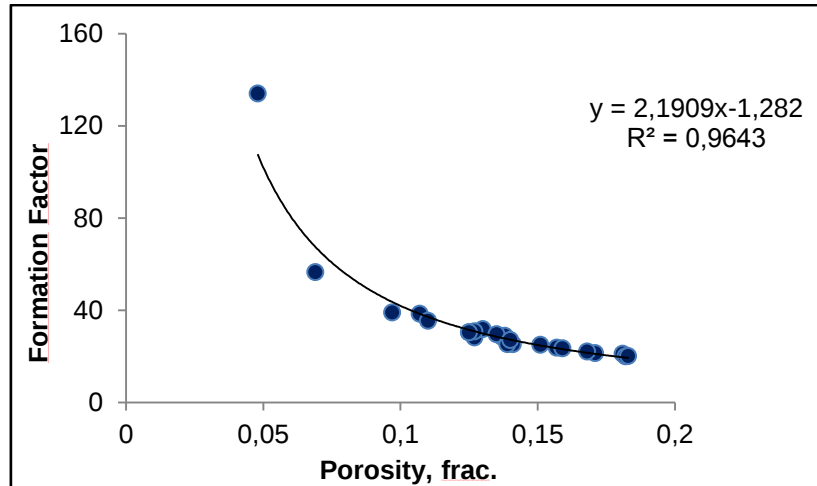
Figure 3.15 Formation Factor vs porosity plot for “a”, ”m” estimation
