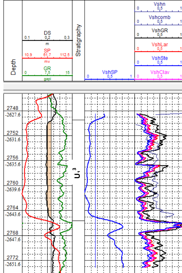
Fig 3.3 Shaliness curves constructed by all considered methods
