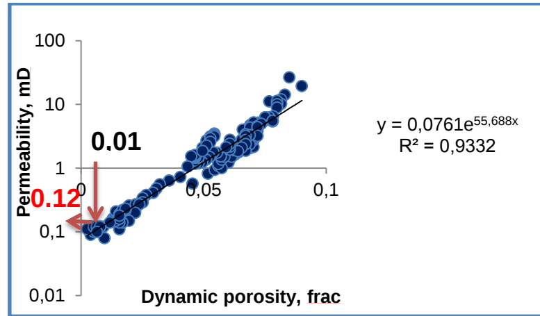
Figure 3.24 Permeability critic value determination
