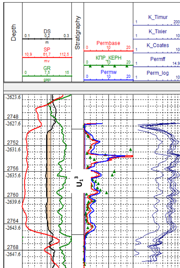
Fig 3.14 Matched and other permeability curves constructed by all considered methods
