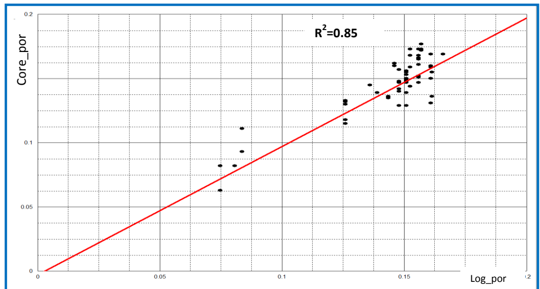
Figure 3.6 Correlation of Neutron effective porosity (SP) vs Core porosity
