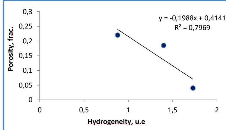
Figure 3.4 NGR units vs porosity relation
