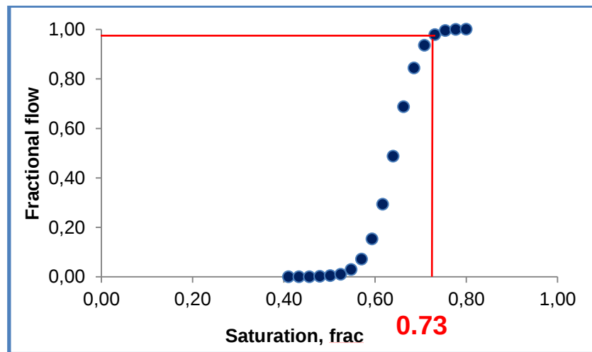
Figure 3.21 Water saturation critical value determinations
