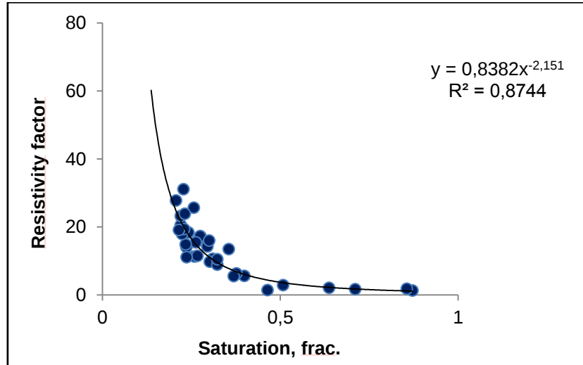
Figure 3.16 Resistivity index vs saturation plot for “n. b” estimation
