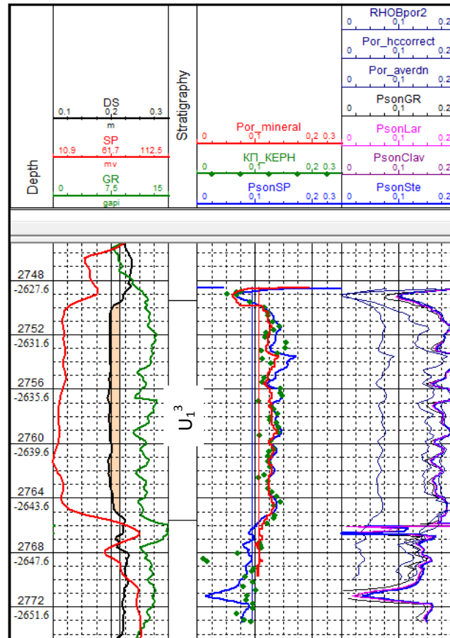
Fig 3.10 Matched and other Porosity curves constructed by all considered methods
