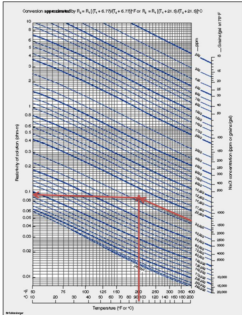
Figure 3.17 Plot for formation water resistivity determination
