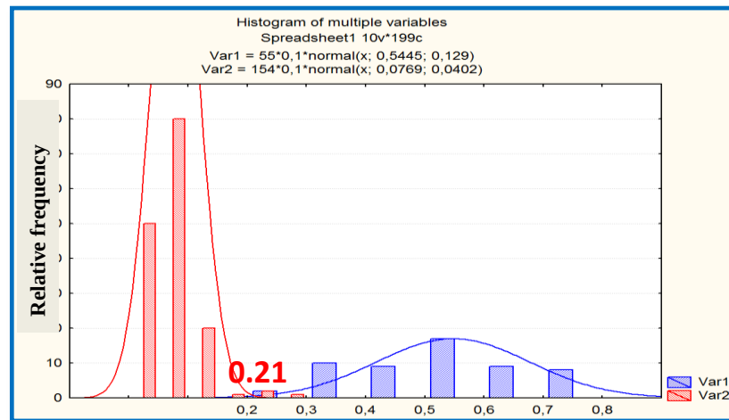
Figure 3.22 Shaliness critic value determination
