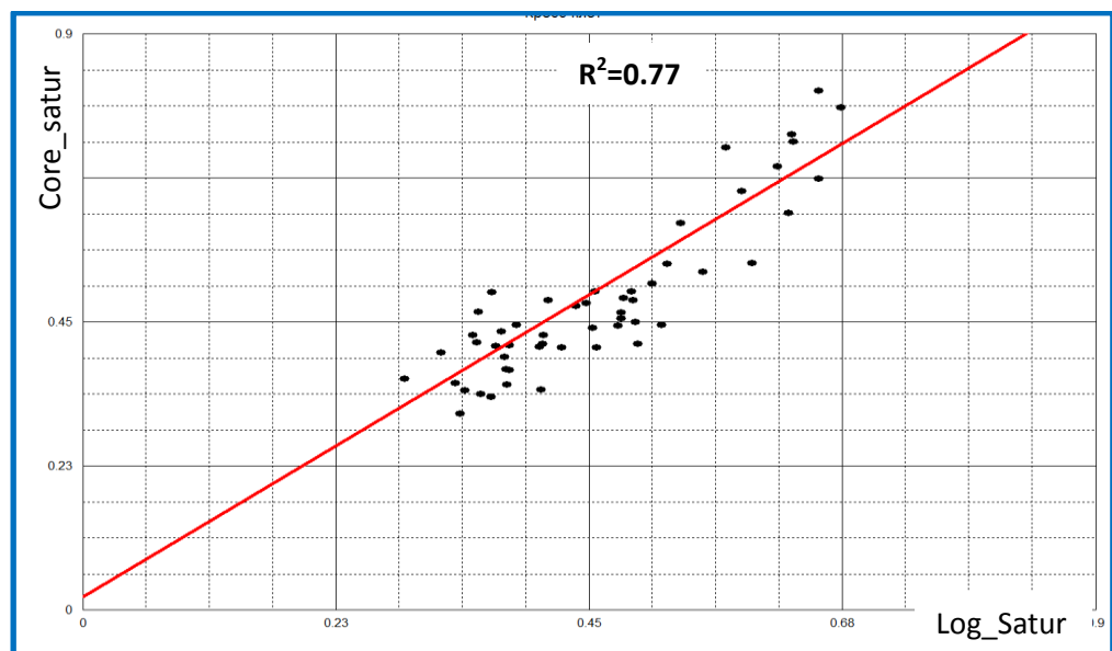
Figure 3.19 Correlation of Total shale model water saturation vs core connate water saturation data
