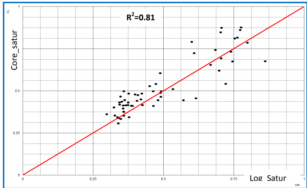
Figure 3.18 Correlation of Archie model water saturation vs core connate water saturation data
