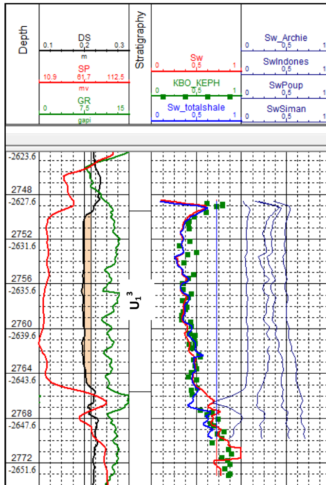
Fig 3.20 Matched and other water saturation curves constructed by all considered methods
