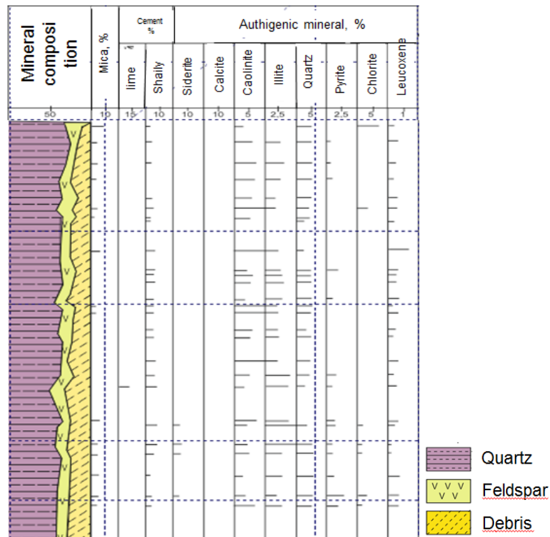
Fig. 3.5 Mineral composition of the core obtained from well № 220
