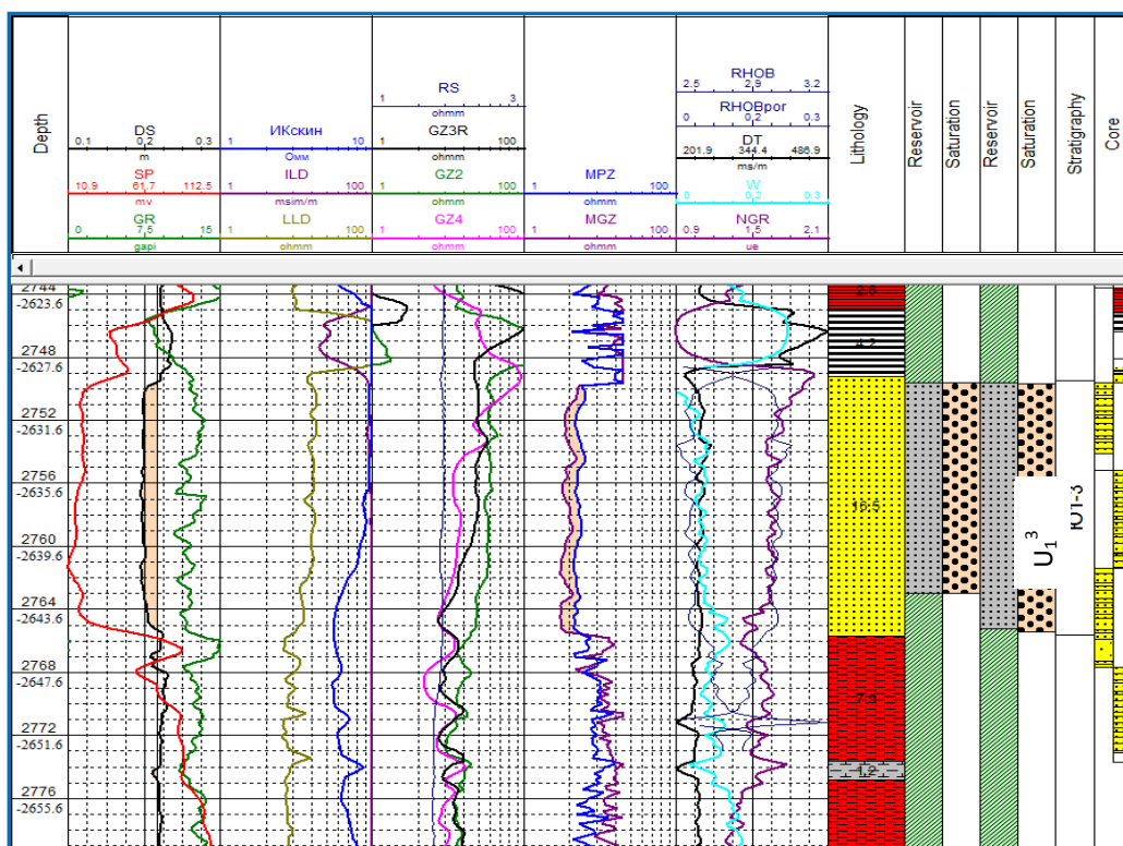
Fig. 3.1 Sketch board of 220 well
