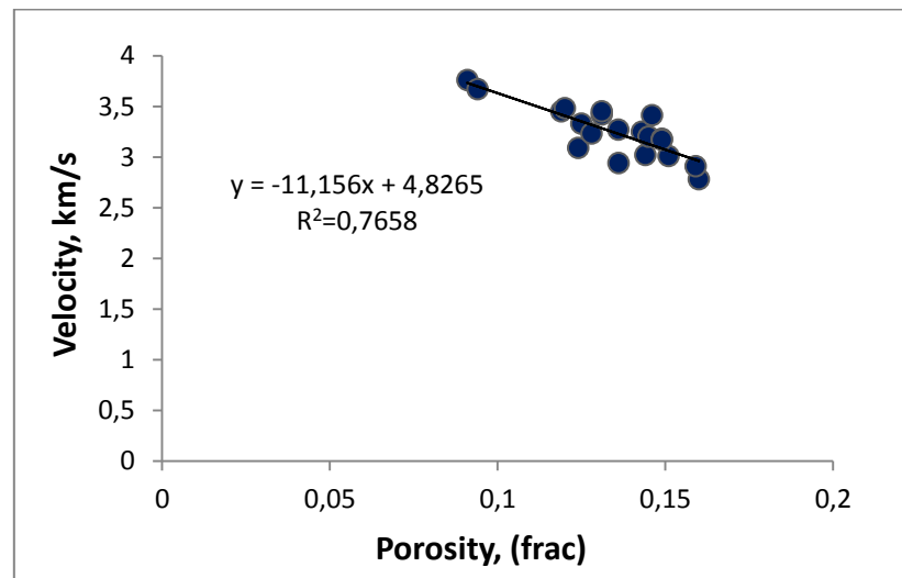
Figure 3.7 Wave velocity vs porosity relationship
