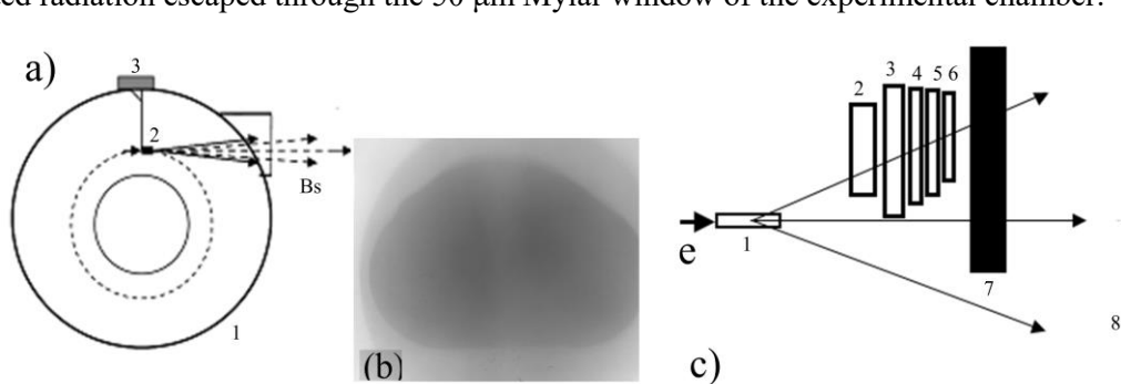
Figure 1. The experimental scheme: a) 1 – betatron chamber (view from above), 2 – thin target, 3 – goniometer, Bs – Bremsstrahlung; b) Photograph of Bs beam ; c) Layout of steel plates in the beam of microfocus Bs gamma-rays of 18 MeV betatron.
