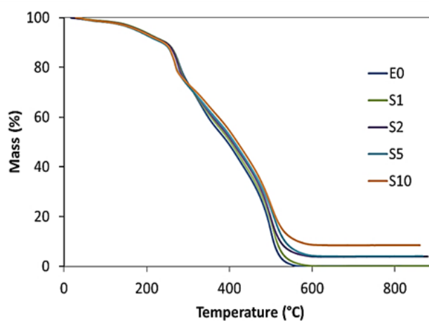
Figure 4. TG curves of epoxy composites filled with zeolite at heating under air.
