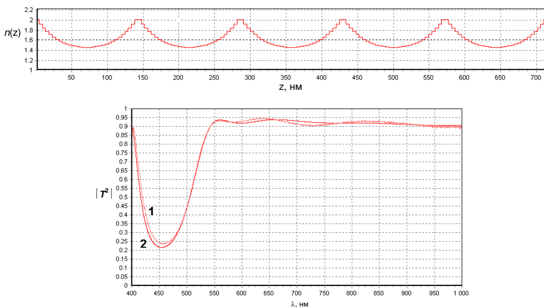
Fig. 1. Nanogradient five-period profile of n(z) for coating from \text{SiO}_2 + \text{Ta}_2\text{O}_5 mixture (the upper plot) and calculated (1) and experimental (2) transmission spectra of the coating (the lower plots). The substrate is from quartz glass
