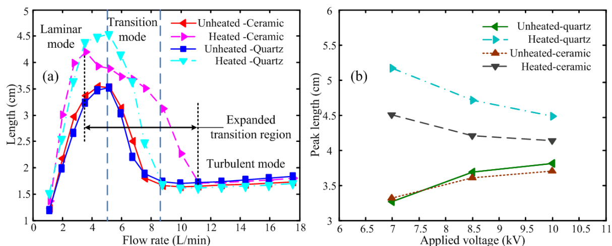
Fig. 1 (a): The plasma plume length versus Ar flow rate at applied voltage of 8.5 kV. (b): The peak length of plasma plume versus applied voltage.
