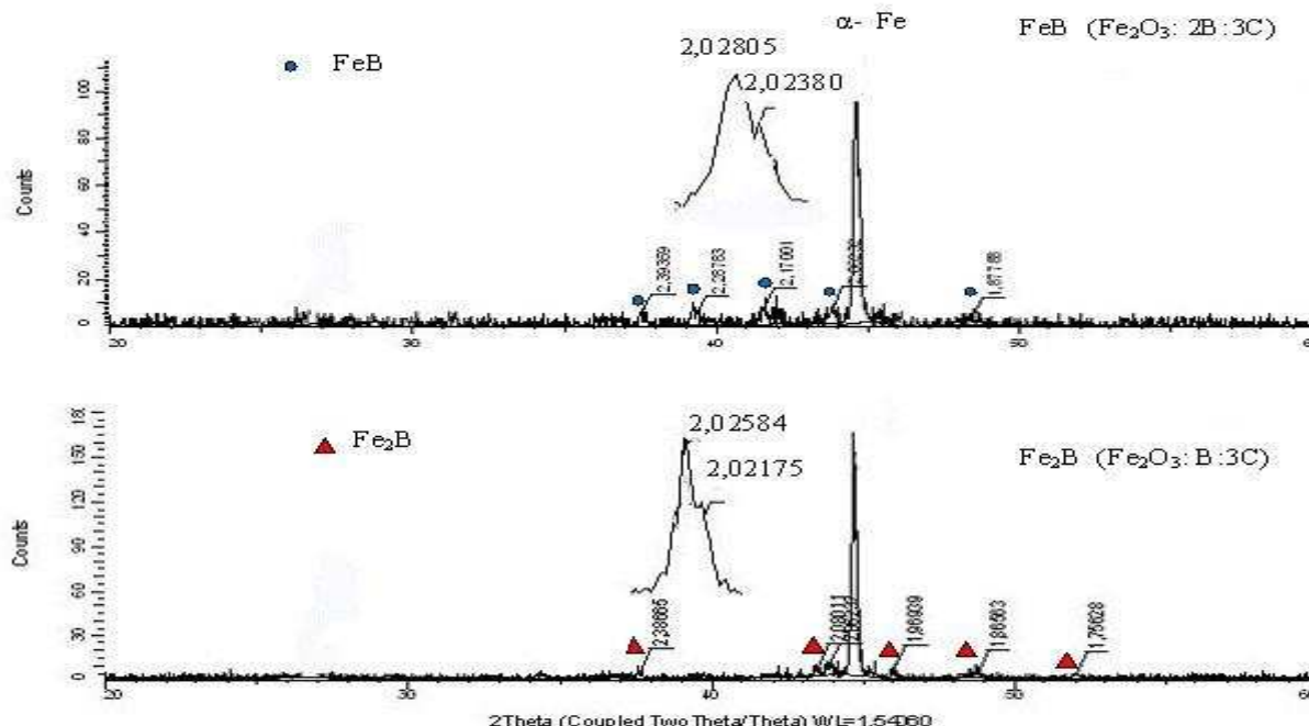
Fig. 1. X-ray phase analysis of produced boride layers
