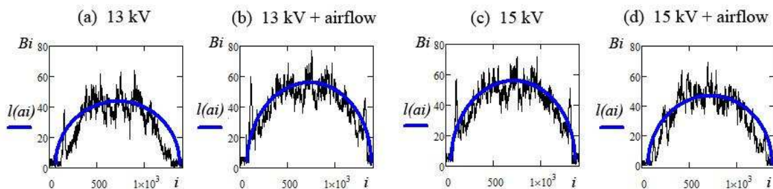
Fig. 2. Distributions of DBD emission brightness in a central layer (10 \mu m) of the DG cross section. 2 mm air gap, P = 1 atm.
