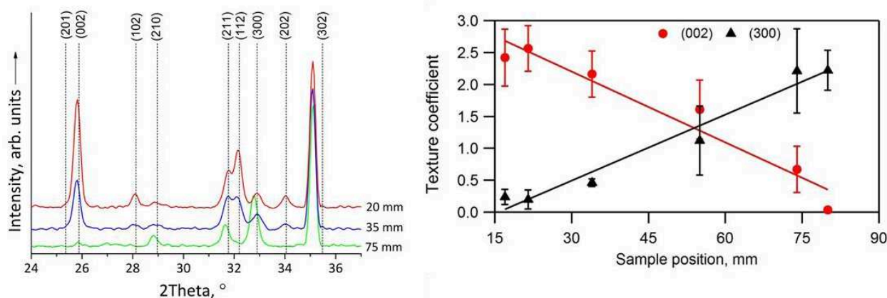
Fig. 1. The XRD patterns of the HA coatings deposited at different sample position on the substrate holder (left) and texture coefficient variations of (002) and (300) planes as a function of sample position relative to the center of substrate holder (right).
