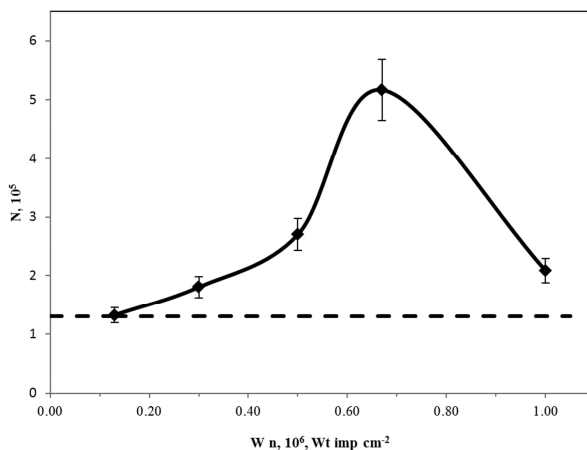
Fig. 1. Dependence of an average (averaging performed on five samples) number of cycles N to failure of silumin on the product of the W_s energy density and the number of pulses of n electron beam treatment. The values of fatigue life of the initial material are shown by the dotted line.
