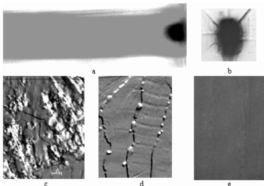
Fig. 1. a - the channel 1 cm length, 200 microns wide, induced by femtosecond laser pulses in NaF (a dark spot on the right – the self-focusing area coinciding with geometrical focus); b – cross section of the channel in NaF (geometrical focus on a crystal surface); c, d – destructions in focal area made by femtosecond laser pulses in LiF crystal; e – unirradiated LiF
