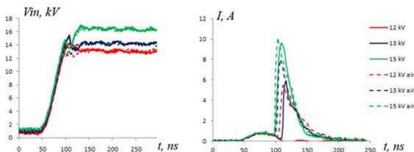
Fig. 1. Waveforms of the voltage applied to the electrodes of the DG and corresponding current discharge pulses for two cases: with airflow (dotted line) and without it (solid line) at different voltage amplitudes of DC power supply [2], 2 mm-air gap, P = 1 atm.
