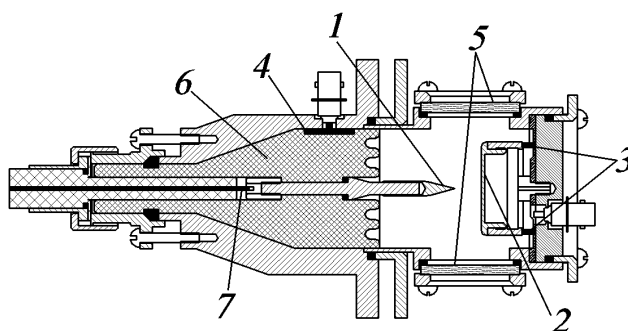
Fig. 1. Scheme of the working chamber: (1) cathode No1, (2) anode, (3) chip resistor shunt, (4) capacitive divider, (5) quartz windows, (6) insulator, and (7) high-voltage cable.
