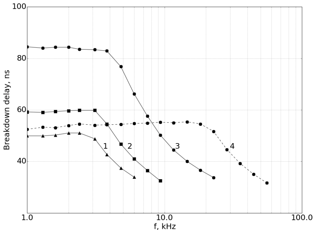
Fig. 1. Dependence of breakdown delay of the switch with 1mm inter-electrode distance on frequency. U = 11 kV; P_{He} = 10 Torr (1), 8 Torr (2), 6 Torr (3,4); P_{H_2} = 0 Torr (1-3), 0.2 Torr (4).
