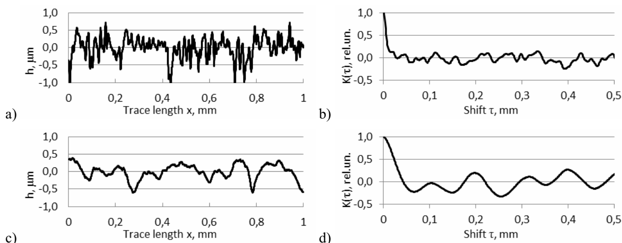
Fig. 1. Profilograms (a, c) and autocorrelation functions (b, d) from the outer surface of the samples after mechanical polishing (a, b) and ion-beam treatment (c, d)
