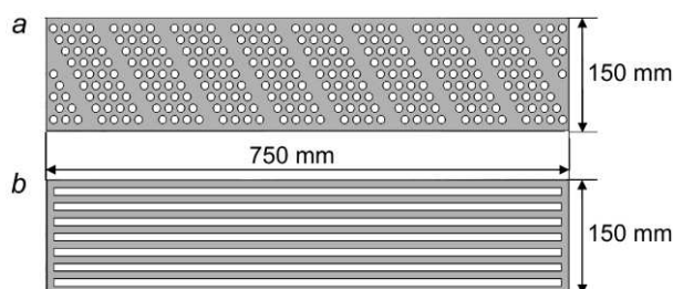
Fig. 2. Mask geometries
