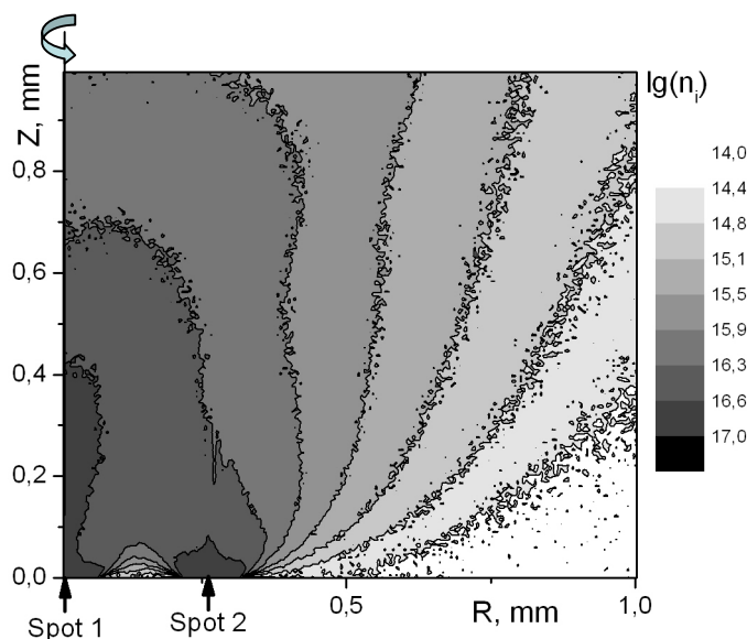
Fig. 1. An example of quasistationary ion density distribution in the case of mixing of jets coming from spot1 and ring-shaped spot2, that mimic the group-spot; [density] – \text{cm}^{-3} , total current 500 A.
