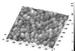
Fig. 2 The silver nanoparticles on the Si. AFM.
