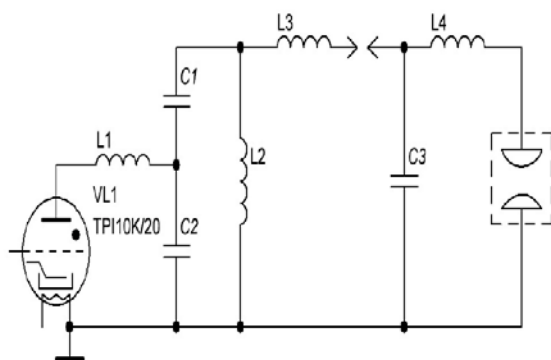
Fig.1. Schematic diagram of excitation circuit. C1= 80 nF, C2= 40 nF, C3= 22 nF, L1= 20 nH, L2= 0.15 mH, L3= 150 nH, L4 = 3 nH
