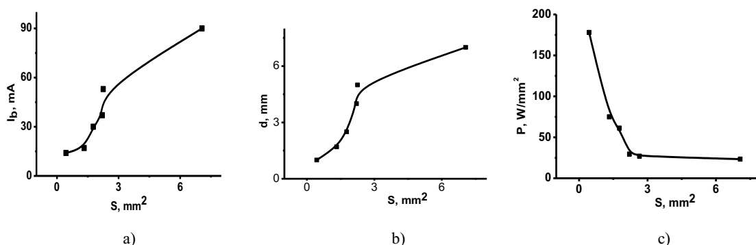
Fig. 1. Dependence of a e-beam current a), diameter of the focused electron beam b), measured in its focal plane, and the power density delivered to the target c), depending on the area of an anode emitting surface, at accelerating voltage of 10 kV, discharge current 500 mA, and pressure 9 Pa.
