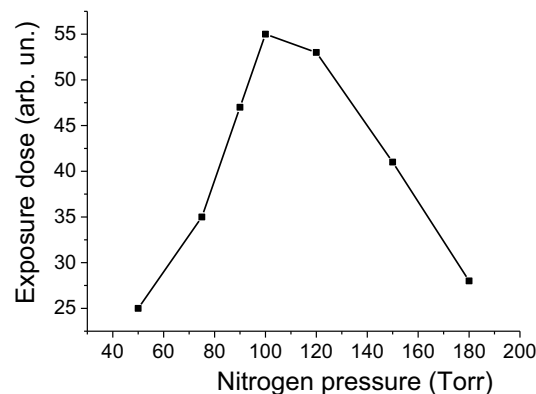
Fig. 1. X-ray exposure dose as a function of the nitrogen pressure in the experiments performed with the sharpening spark gap.
