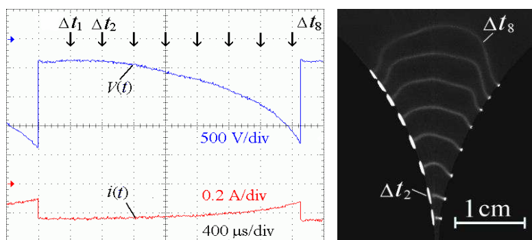
Fig. 1. Voltage and current waveforms jointly with CCD frames are used for estimation the parameters of gliding glow discharge.
