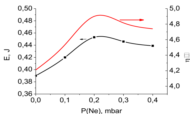
Fig. 1. Dependence of the output radiation energy and laser efficiency as a function of Ne pressure in the gas mixture.
