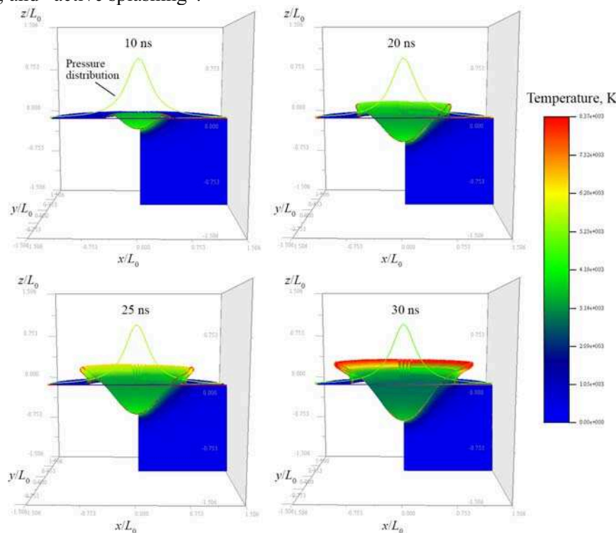
Fig. 1. Results of simulation of the crater and jet formation for a pressure P = 4 \cdot 10^8 Pa exerted by the reactive force.
