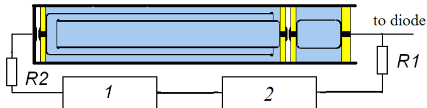
Fig. 2. The schematic of the trigger pulse formation for external triggering of the main spark gap: R1 and R2 – resistance of a voltage divider and a resistance limiting the current through the discharge gap, respectively; 1 – transformer; 2 – a cable used for the formation of a delay time between formation of a trigger pulse and arrival of this pulse to the trigger electrode of the trigatron spark gap
