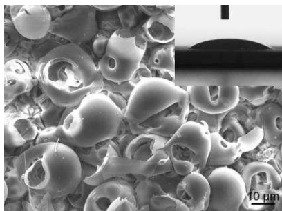
Fig. 1. SEM micrograph of CaP coating with image of water drop on surface produced at oxidation voltage of 200 V.
