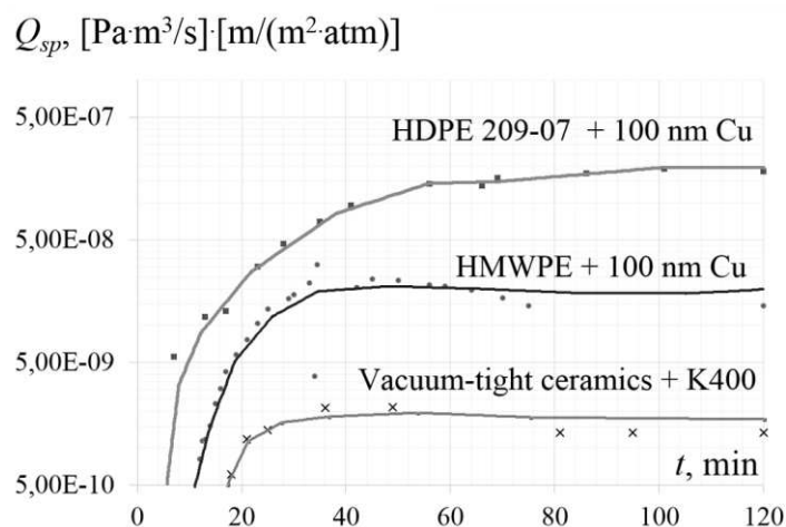
Fig. 1. Helium permeation through materials for gas discharge plasmas devices
