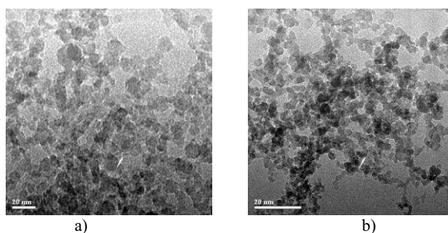
Fig. 1. TEM images of nanoparticles produced by spark discharge: a) \text{Al}_2\text{O}_3 ; (b) Fe oxide.
