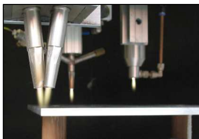
Fig. 1. Different atmospheric plasma jet systems usable for APCVD of composite coatings
