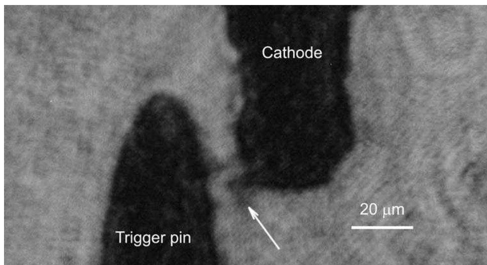
Fig. 1. Picture of dense plasma object (arrowed) at the cathode taken with CCD camera (open shutter, effective exposure is equal to laser pulse duration – 20 ns). Arc current 25 A.
