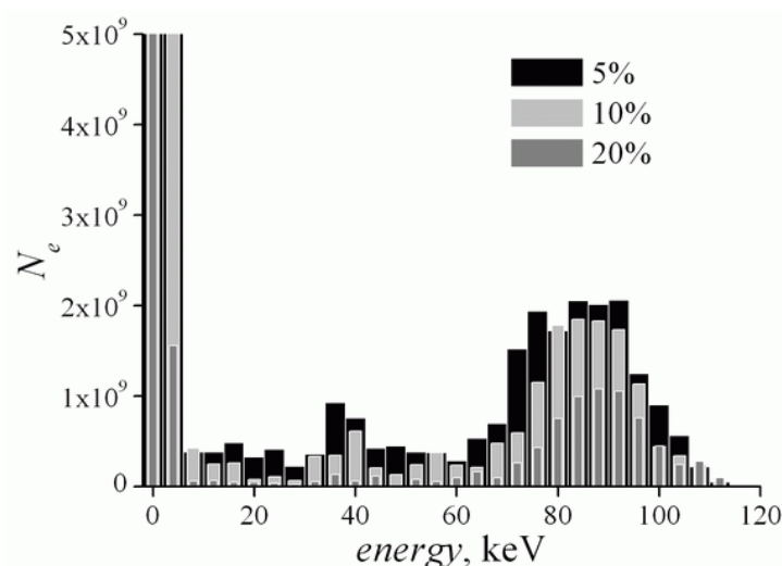
Fig. 1. Electron energy distributions for different concentrations of neutral molecules in hot region. (percentage of molecule concentration in surrounding gas media)
