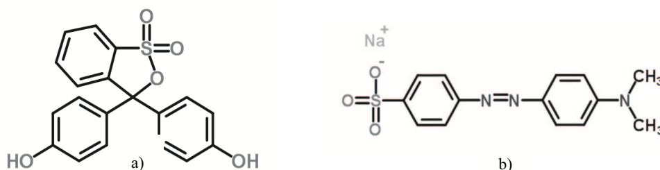
Fig. 1. Chemical structures of phenol red (a) and methyl orange (b) dyes.
