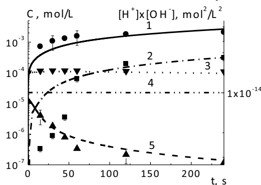
Fig. 2. Kinetics of the phenol red destruction and some products formation: 1 – H 2 O 2 ; 2 – H + ; 3 – Hind; 4 – [H + ][OH - ]; 5 – Ind - . Points – experiment, lines – calculation.
