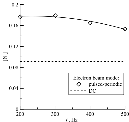
Fig. 1. Time-averaged atomic nitrogen ions content in the total ion flux sampled from beam plasma depending on the electron beam current pulse frequency and in DC-mode (for comparison).
