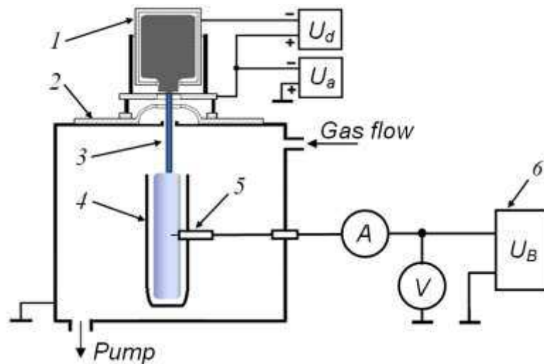
Fig. 1: Experimental apparatus: 1 – fore-vacuum plasma electron source, 2 – vacuum chamber, 3 – electron beam, 4 – dielectric cavity, 5 – Langmuir probe, 6 – probe bias voltage supply U_B . U_d , U_a – discharge and accelerating voltages power supplies, respectively.
