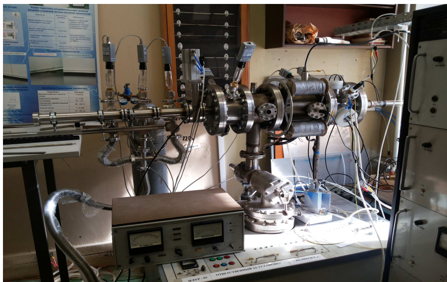
Fig. 1. Instalation ILUR-03
