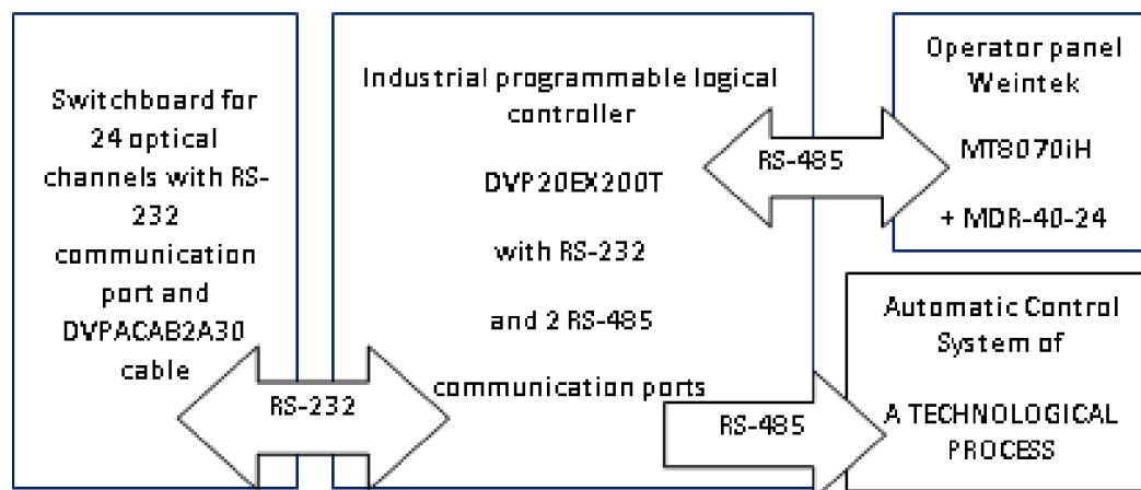
Fig. 1. The symbolic scheme of the communication module for 24 channels AP system control.
