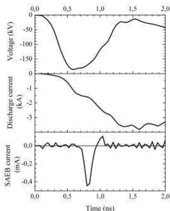
Fig. 1. Waveforms of voltage pulses (a), current through gap (b) and runaway electron beam behind foil (SAEB) (c). d = 13 mm. Pressure of SF 6 : 0.05 MPa.
