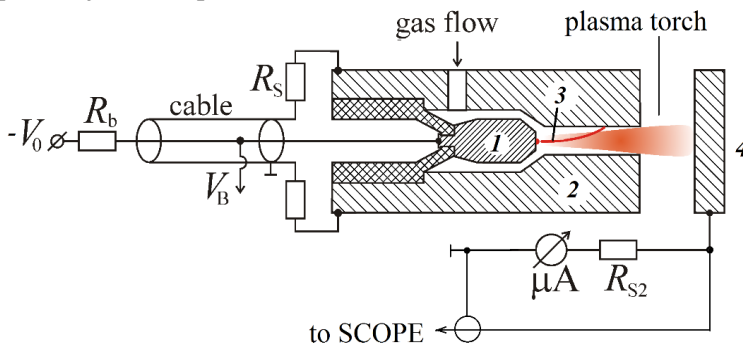
Fig. 1. Schematic of the low-current nonsteady state plasmatron for obtaining the plasma jet (plasma torch) in air. 1 – cathode of the plasmatron, 2 – anode nozzle, 3 – plasma column, 4 – probe for measuring a current flowing via the plasma torch, V_0 – voltage of dc power supply, R_b – ballast resistor, R_s – current shunt for recording a current to the anode nozzle, R_{s2} – current shunt for recording a current to the probe.
