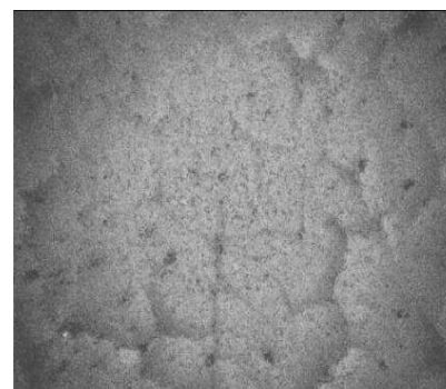
Fig. 2. Microstructure of TiN-Cu layer
