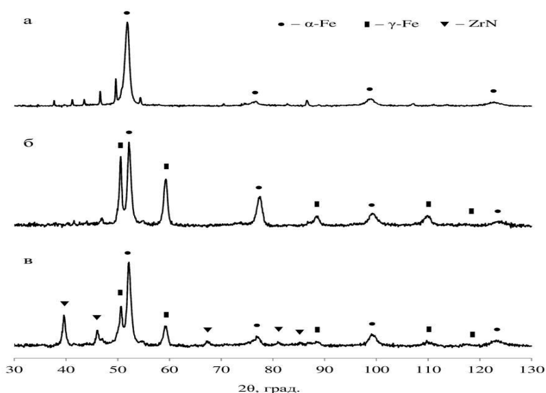
Fig. 1 a) diffraction pattern (CoK \alpha ) from a surface of the nitrated high speed cutting steel P6M5 б) the same after the influence of wide-aperture low-energy high-current electron beam, в) the same after zirconium microalloying.
