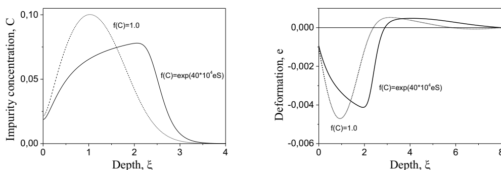
Fig. 1. Influence of the function f(C) form on the distribution of the implanted impurity and deformation wave. Times, \tau = 8.0 .
