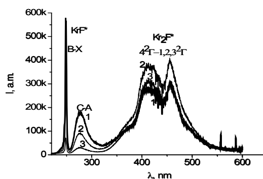
Fig. 2. The emission spectrum of the discharge. Mixture: Ar/Kr/F 2 = 1000/400/1 mbar, P = 1.4 bar, U 0 = 25 kV. The opening of the optical shutter for the time of discharge: 1– 0-50 ns; 2– 50-100 ns; 3–100-150 ns.
