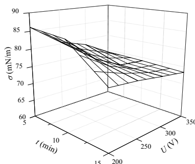
Fig. 2. 3D-plot of the free surface energy of CaP coatings against the oxidation voltage and duration.
