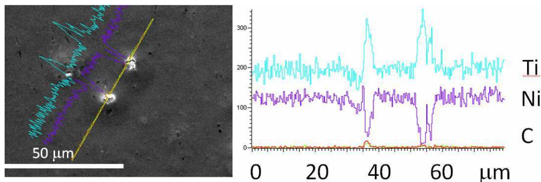
Fig. 1. SEM image of the surface of irradiated TiNi (backscattered electrons). On the right the line microanalysis of chemical composition is presented.
