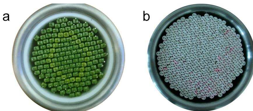
Figure 1. Explosive-emission cathode with resistive decoupling of the emitters: cathode based resistors TBO-1 (a); the cathode made of Ni-Cr wires inserted into ceramic tube (b).
