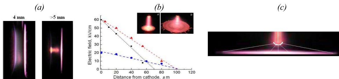
Fig. 1. (a) Images of the diffuse and constricted helium APGD at a current of 1 A; (b) Longitudinal electric field profiles in a cathode fall for cooled (squares, inset a above) and uncooled (triangles, circles, inset b above) cathodes. Square and triangle symbols correspond to axial profiles, the circles – at a distance of 8 mm from the axis; (c) Spatial profile of currents in cathode region
