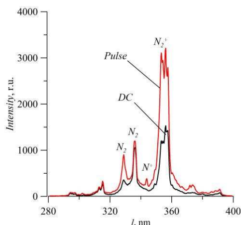
Fig2. Characteristic emission spectra of EBP at DC and pulse-periodic regimes.
