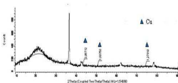
Fig. 1. XRD patterns of TiN-Cu film: d) 60 A (280 mm)
