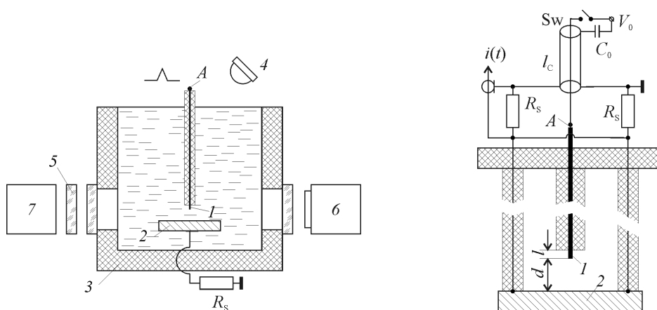
Fig. 1. Schematic of arrangement and sketch of electrode system: 1 – active electrode, 2 – return electrode, 3 – case, 4 – lighter, 5 – filter, 6 – camera, 7 – photomultiplier. C_0 = 40 \mu\text{F} , R_s = 0,01 \Omega .
