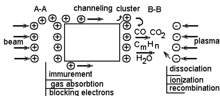
Fig. 1. Model of the interaction of the ion flux to the crystal
