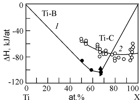
Fig. 1. The enthalpy of compound formation in systems Ti-B (curve 1) [1] and Ti-C (curve 2) [2] at 298 K
