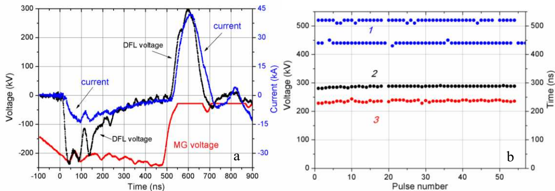
Fig. 1. The waveforms of voltage and current at the output of Blumlein and charging voltage of Blumlein (a). Variation in the duration of the first voltage pulse at different length of the cable (1) and variation in the breakdown voltage of the main gap (2) and the preliminary spark gap (3) operated in externally triggered mode (b)
