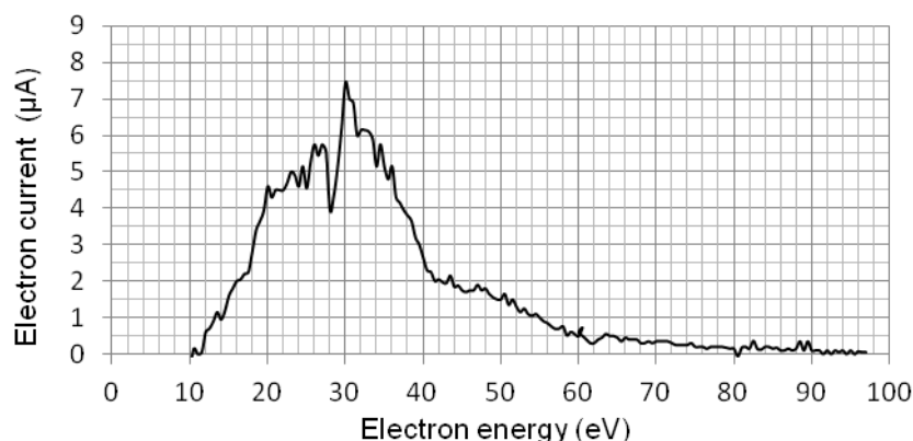
Fig. 1. The distribution of electrons on energy in the ion beam.
