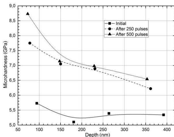
Fig. 1. Dependences of surface microhardness versus its depth for initial stainless steel samples, and samples treated by REP DD.
