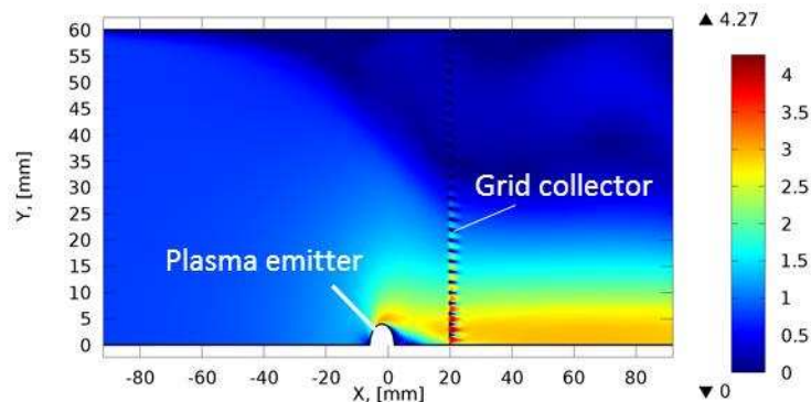
Fig. 1. Numerical simulation results: air velocity as colored surface map with units in m/s
