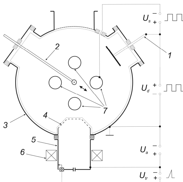
Fig. 1. The scheme of experimental installation. 1- the main discharge anode, 2 – the single cylindrical Langmuir probe, 3 – the vacuum chamber (the main discharge cathode), 4 – the anode of the arc discharge, 5 – the source of arc discharge with the cold hollow cathode, 6 – the magnetic field coil, 7 – samples.
