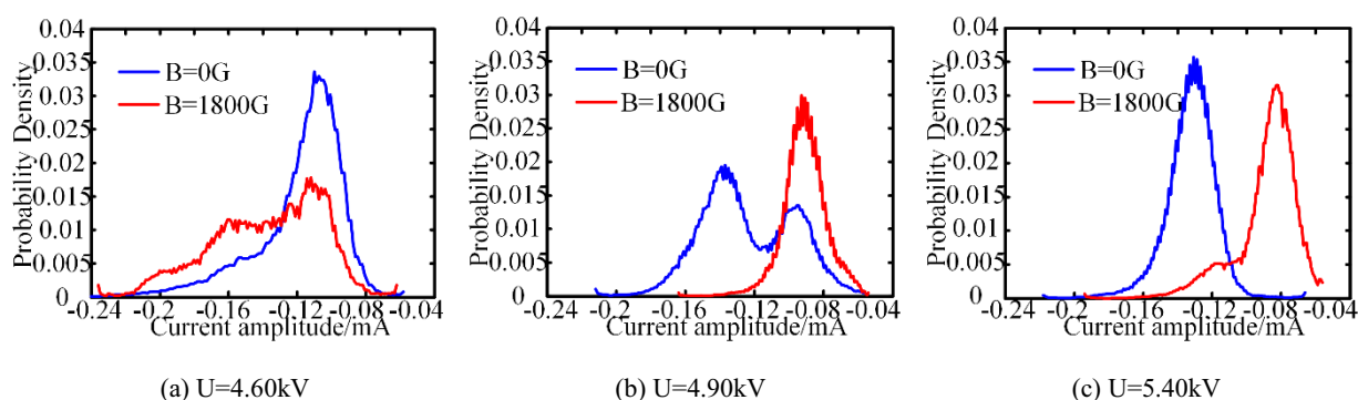
Figure 1 Statistical characteristics of the discharge current amplitude under different voltage
