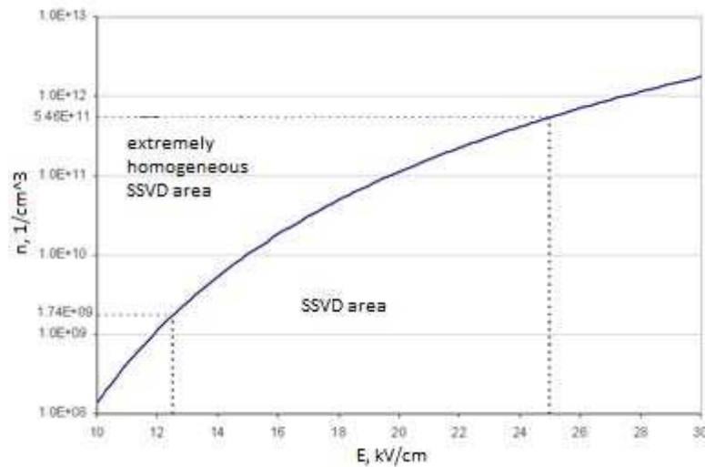
Fig. 1. Calculated dependence of boundary concentration of initial electrons n_0 on the field strength E in the DG for producing extremely homogeneous SSVD in the mix of CO 2 :N 2 :He = 1:2:3 at p = 1 atm.
