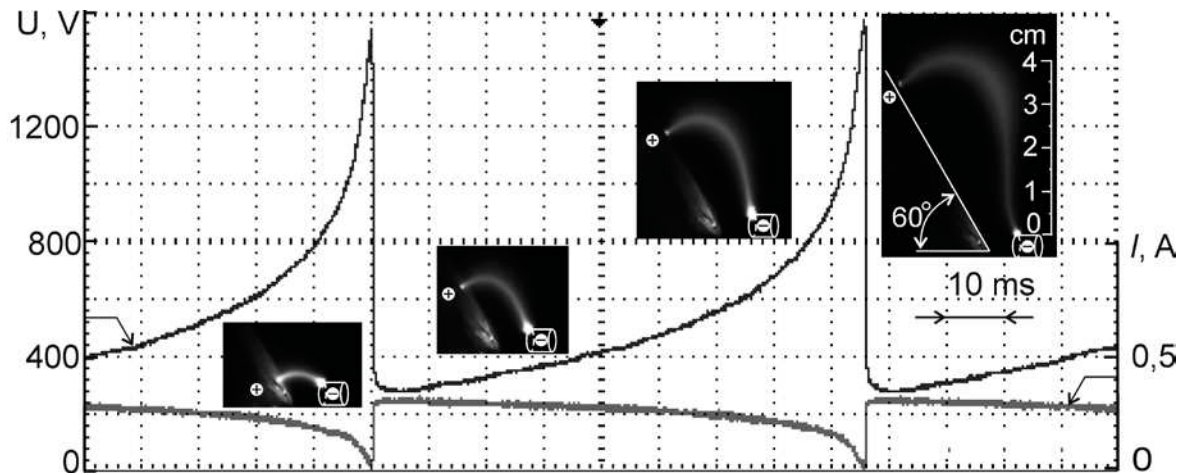
Fig. Oscillograms of voltage and current. Cathode – hafnium, anode - copper plate, the inclination angle of 60^\circ . l = 6 mm.
