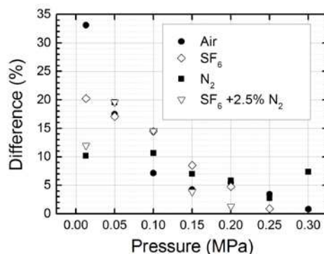
Fig. 1. The differences in the breakdown voltage at positive polarity relatively one at negative polarity in air, nitrogen, sulfur hexafluoride and sulfur hexafluoride with small (2.5%) nitrogen admixture at a pressure range of 0.013-0.3 MPa
