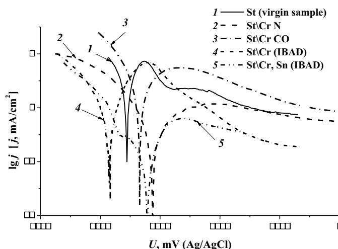
Fig. 1. Current-potential plots in 1M \text{H}_2\text{SO}_4 + 2 \cdot 10^{-6}\text{M} HF solution of stainless steel (St) samples with coatings produced by cathode arc plasma erosion sprayed and with layers prepared by ion beam assisted deposition from vacuum arc discharge plasma
