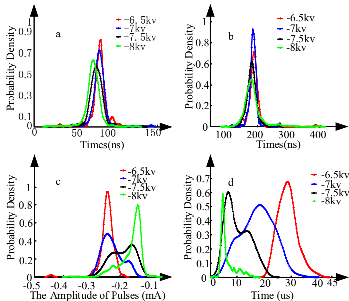
FIG.1 the probability density of parameters. a). the probability density of the rising time. b). the probability density of the falling time. c). the probability density of the amplitude of pulses. d). the probability density of the interval of pulses
