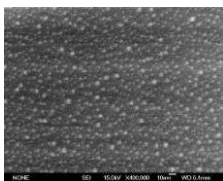
Fig. 1. The surface of the silver nanofilms. SEM.
