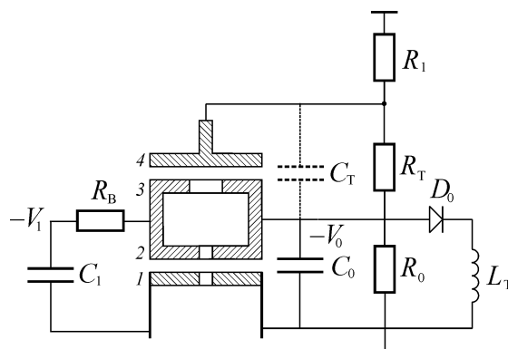
Fig. 1. Design of electrode system and electric circuit for investigation of recovery of the main gap. C_T is the spurious capacitance of the gap 3 – 4; C_0 = 1 nF, R_0 = 70 k \Omega , R_1 = 100 k \Omega , R_B = 10 k \Omega , R_T can be varied from 100 k \Omega to R_T = \infty .
