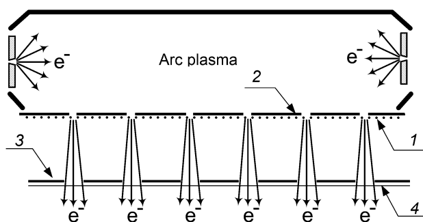
Fig. 1. Scheme of electron source with plasma emitter: 1 – emission grid, 2 – mask, 3 – support grid, 4 – foil
