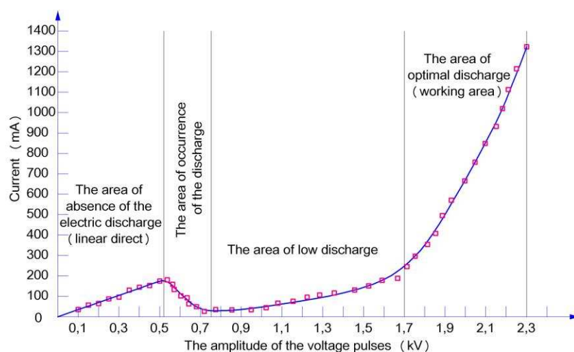
Fig. 1. The volt-ampere characteristic of the diaphragm of the electric discharge
