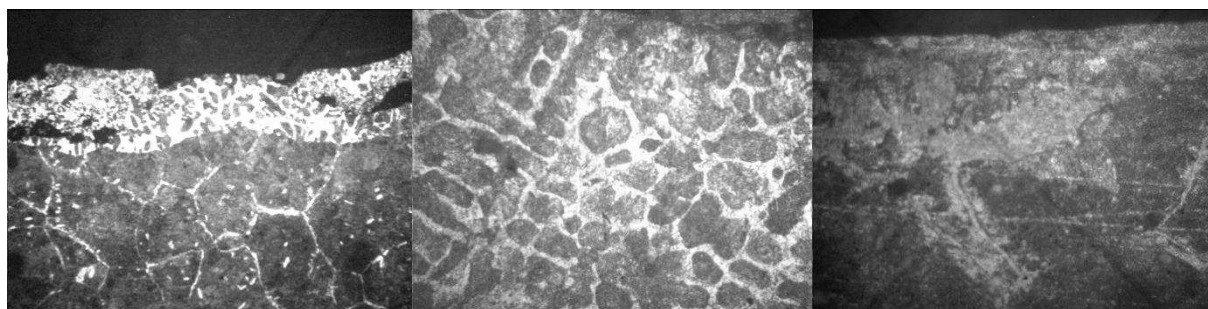
Fig.1. Microstructure of samples ( \text{TiO}_2\text{-B-C} + \text{B}_2\text{O}_3 ) after pulse electron beam processing
