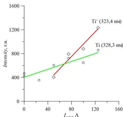
Fig.2. Dependences of Ti and Ti + lines intensities on discharge current pulse amplitude.
