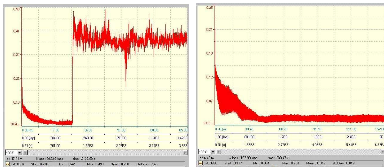
Fig. Friction coefficient \mu of the ultrafine alloy VT6 coating by conventional magnetron sputtering techniques (a) and by the combined magnetron-plasma method with an assistant gas- plasma generator PINK (b)
