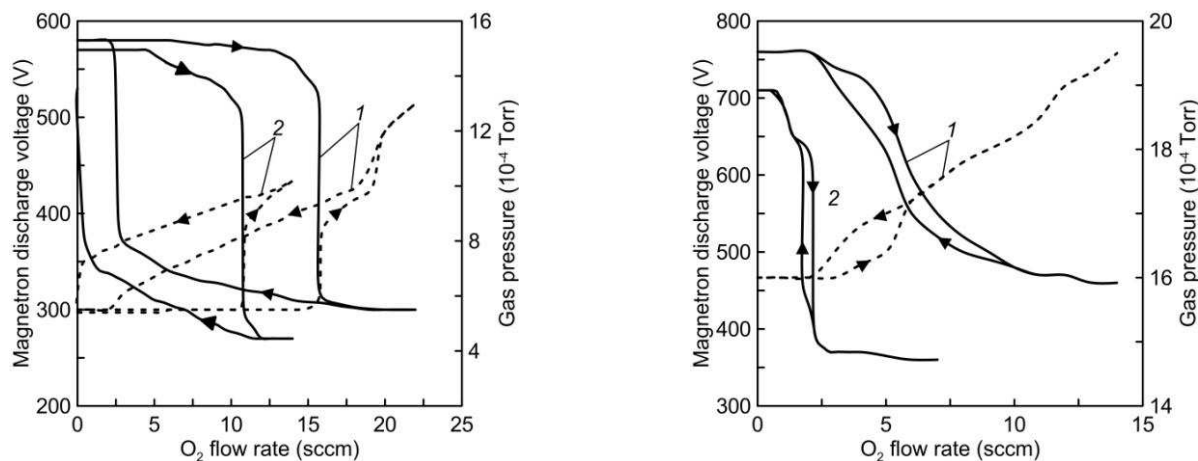
Fig. 1. Dependences of magnetron discharge voltage (solid) and gas pressure (dashed) on O 2 flow rate. Pulse DC (a) and HiPIMS (b) regime. 1 – self-maintained discharge, 2 – mode with electron beam injection, beam current 2 A (a) and 10 A (b).
