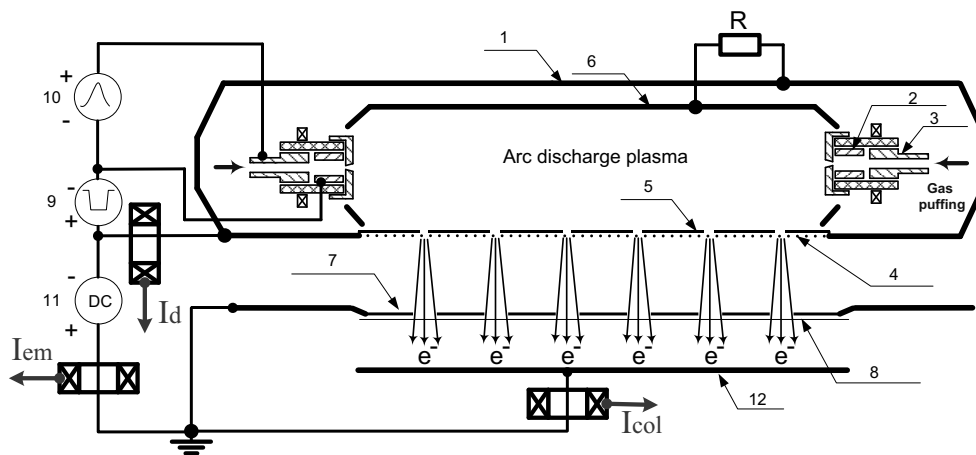
Fig. 1. Scheme electron source with wide-aperture plasma emitter: 1 – hollow anode; 2 – cathode; 3 – igniter; 4 – metallic mesh; 5 – a mask; 6 – screen; 7 – support grid outlet foil windows; 8 – output foil; 9 – discharge power supply; 10 – source power igniter; 11 – high voltage power supply; 12 – the collector.
