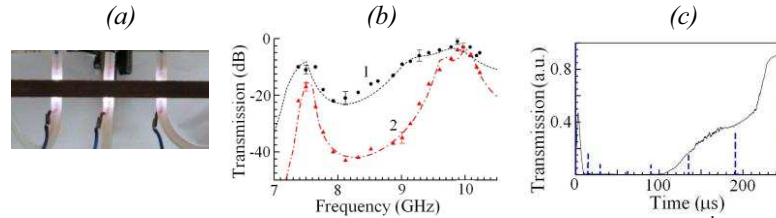
Fig. 1. (a) Image of waveguide section with discharges, (b) transmission spectra at 3 rd (1) and 17 th (2) microseconds and (c) transmission of high power (50 kW) pulses at frequency of 9.15 GHz.
