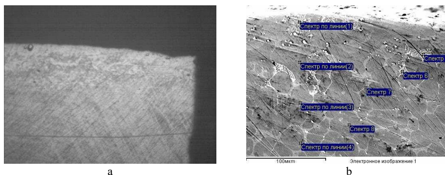
Fig.1. General view (etched layer) (a) and structure (b) layer VB_2 on steel U8A
