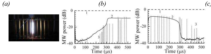
Fig. 2. (a) Image of 2D EBG metallic structure with a discharge column and its transmissions of high power pulses at frequency of 9.15 GHz in a direction of 45^\circ in the cases of defect compensator (b) and additional defect (c).
