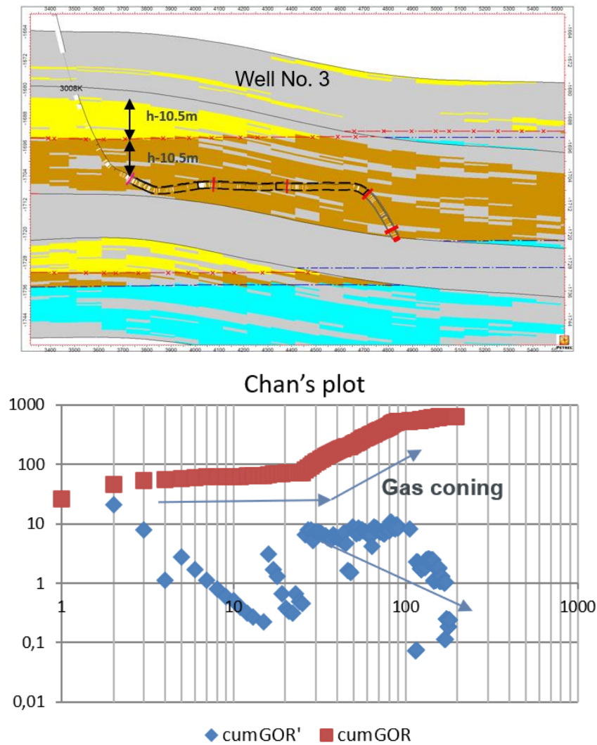
Figure 2 – Well column No. 3 and the Chan's plot Chan's plot for this well indicates the gas coning (Figure 2).
