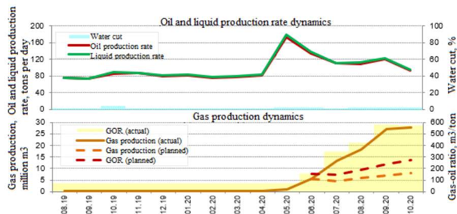
Figure 1 – Oil, liquid and gas production rate dynamics
