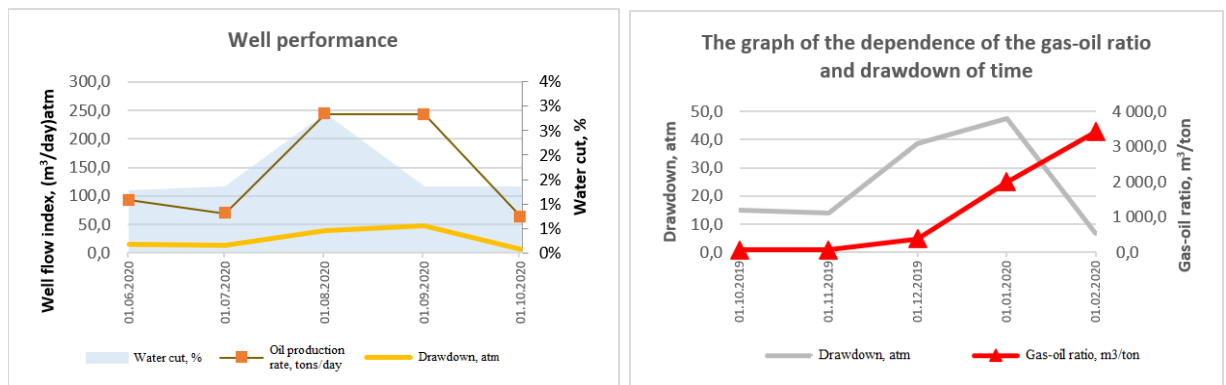
Figure 5 – Operating parameters graphs of the well No. 7
