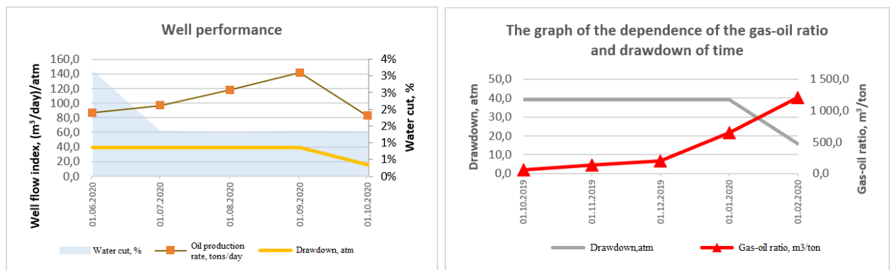
Figure 11 – Operating parameters graphs of the well No. 10
