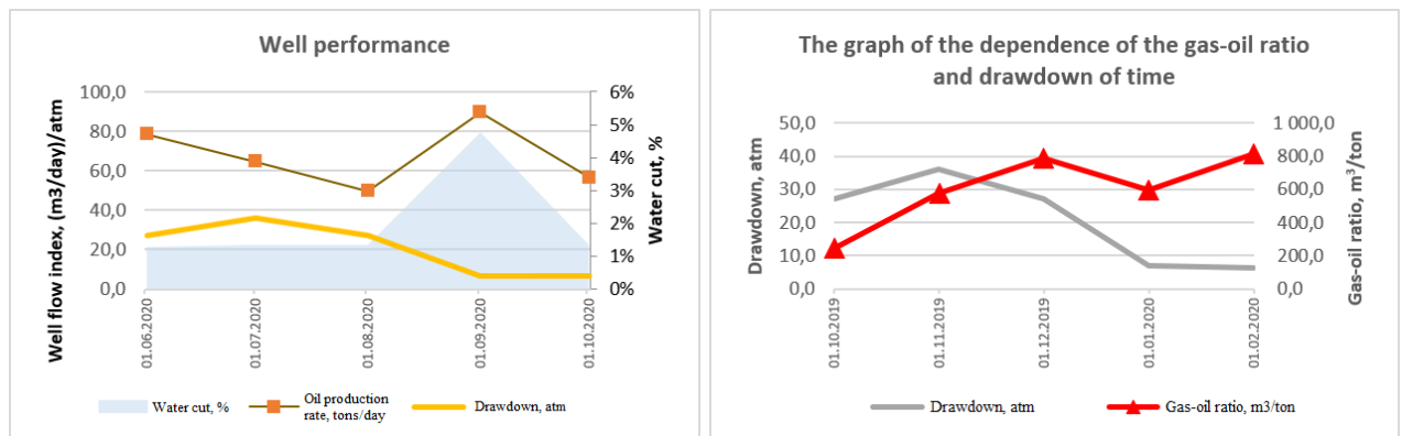
Figure 9 – Operating parameters graphs of the well No. 9
