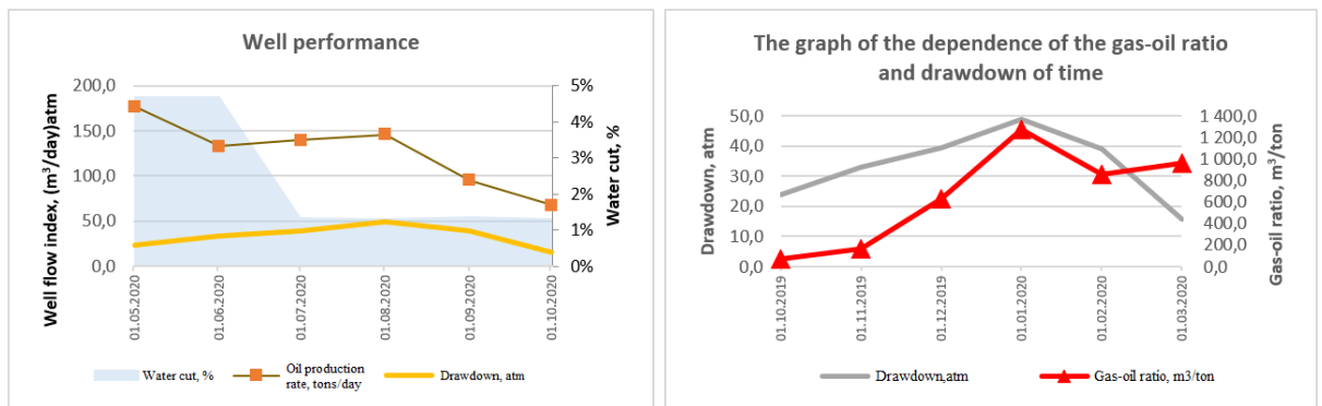
Figure 7 – Operating parameters graphs of the well No. 5
