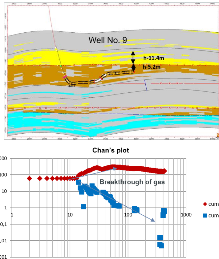
Figure 8 – Well column No. 9 and the Chan's plot
