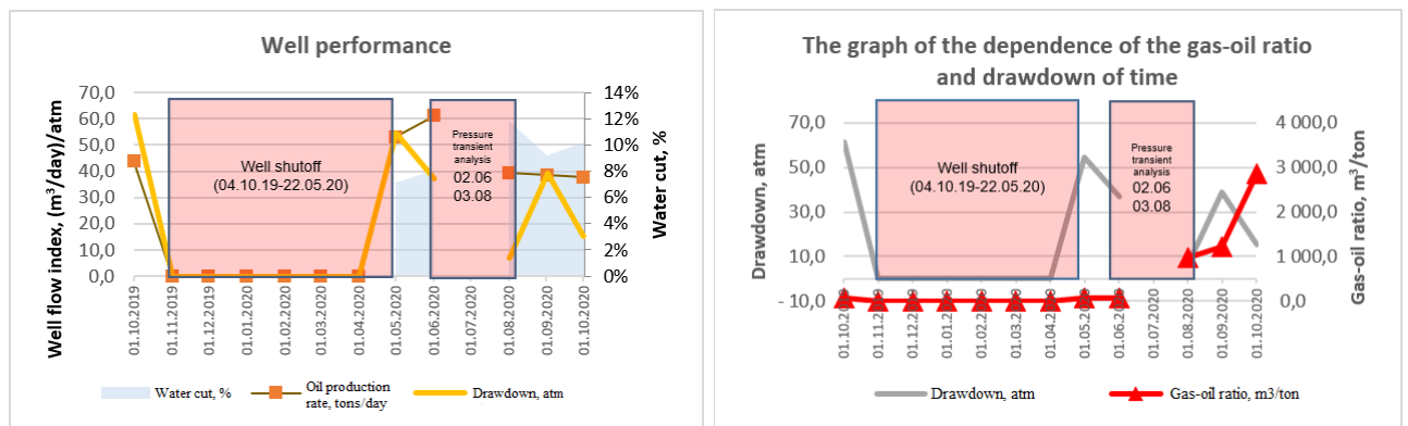
Figure 13 – Operating parameters graphs of the well No. 4
