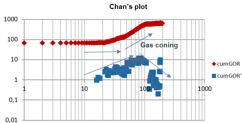
Figure 6 – Well column No. 5 and the Chan's plot
