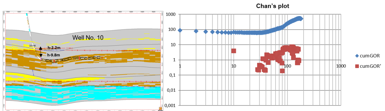
Figure 10 – Well column No. 9 and the Chan's plot
