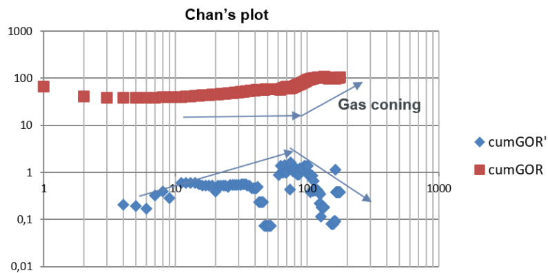
Figure 4 – Well column No. 7 and the Chan's plot
