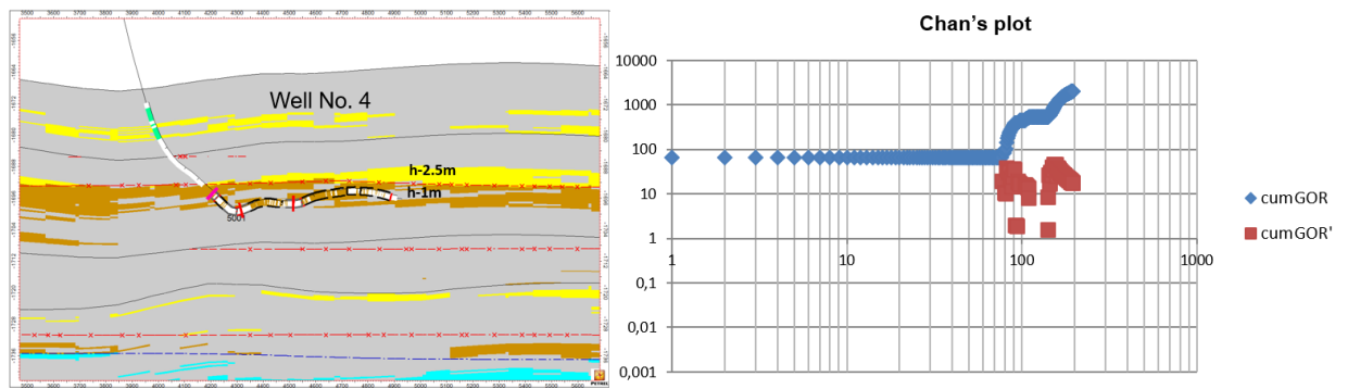
Figure 12 – Well column No. 4 and the Chan's plot
