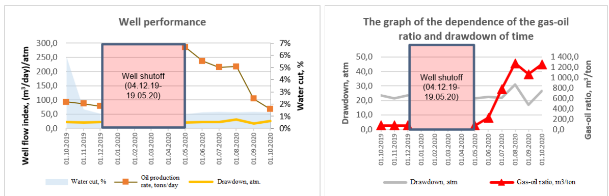
Figure 3 – Operating parameters graphs of the well No. 3
