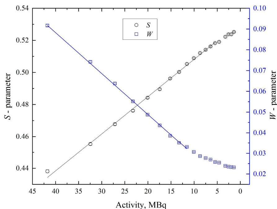
Figure 7. Dependence of S- and W-parameters of DBS on the activity of ^{64}\text{Cu} source.
