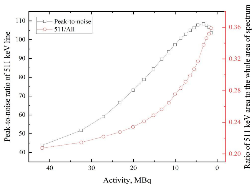
Figure 6. Dependences of 511 keV line peak-to-noise ratio and the ratio area under the line to the area of the whole spectrum on ^{64}\text{Cu} isotope activity.
