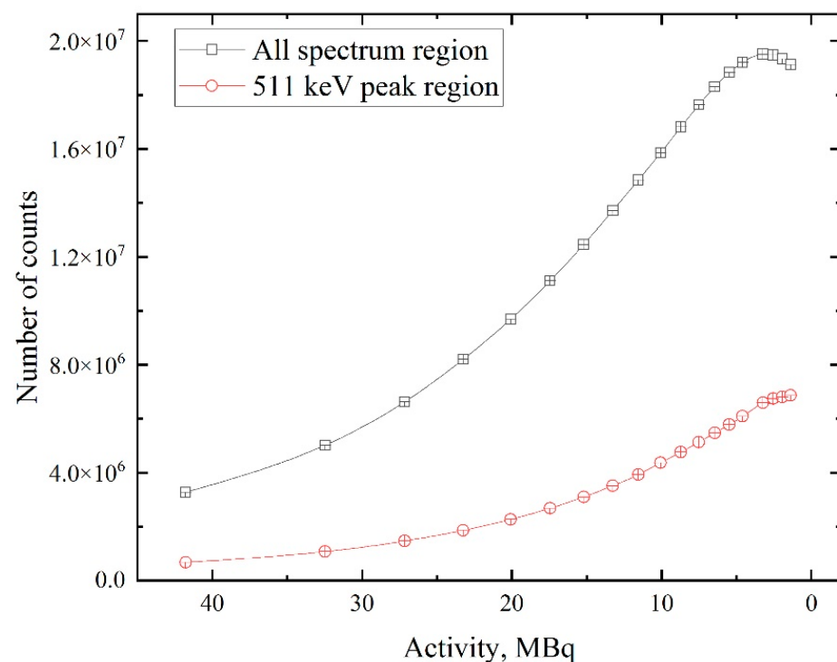
Figure 5. Dependence of the total number of counts in the whole spectrum of ^{64}\text{Cu} isotope and in the range of positron annihilation line (511 keV) on the activity.
