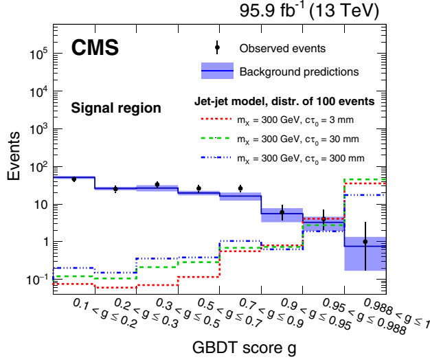
FIG. 6. The predicted background yields and the number of observed events for the data in the signal region, with N_{\text{tracks}}^{3D} smaller than 3 for both jets, shown for different bins of the GBDT scores. The background predictions in different bins are correlated, since the events that are used for background predictions in lower bins are also used in the background predictions in higher bins. For comparison, three benchmark signal points are also shown (dashed lines) for the jet-jet model with m_X = 300 GeV and different lifetimes. For visualization purposes, each signal process is given a cross section that yields 100 events produced in the analyzed data sample.
