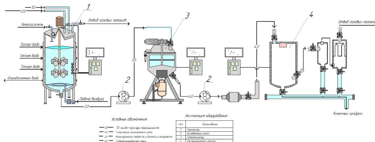
Fig. 1. Machine-hardware scheme for obtaining the product
