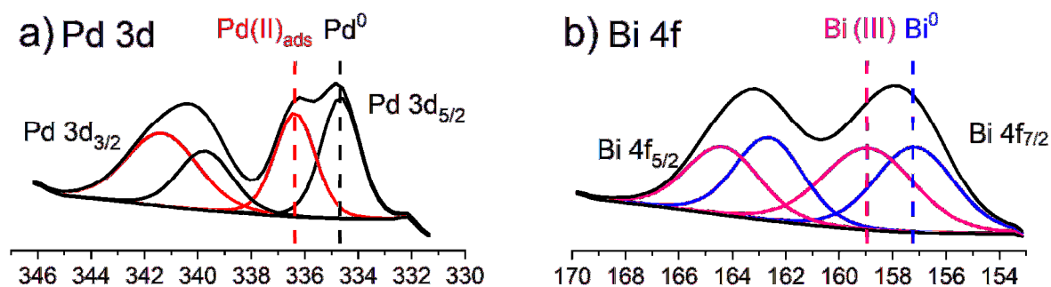
Fig. 2. XPS patterns of the Pd 3d (a) and Bi 4f levels on the PdBi/Al 2 O 3 catalyst surface
