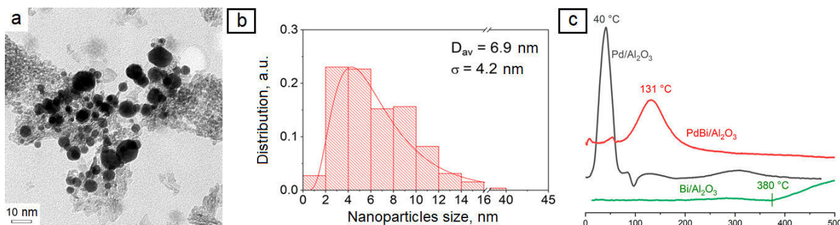
Fig. 1. TEM image (a), particle size distribution histogram (b), TPR pattern of Pd-Bi/Al 2 O 3
