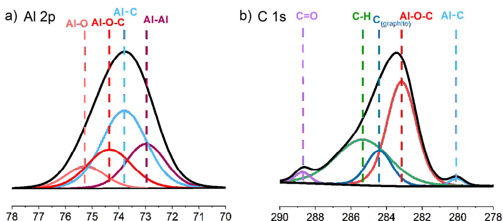
Fig. 3. XPS patterns of the Al 2p (a) and C 1s levels on the PdBi/Al 2 O 3 catalyst surface
