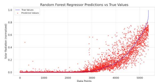
Fig. 2. RFR predictions vs true values (Model 1)
