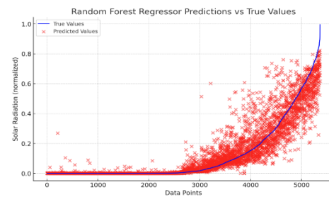
Fig. 4. RFR predictions vs true values (Model 2)
