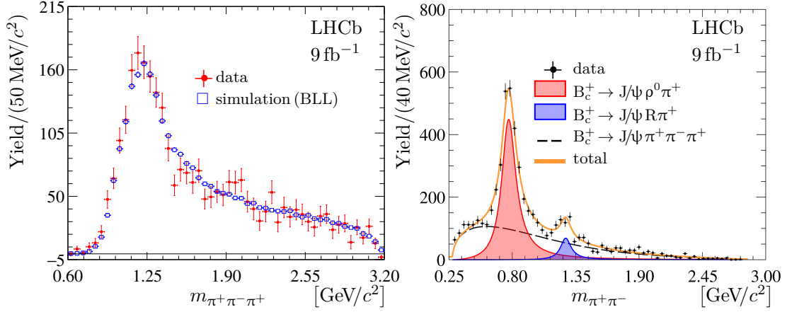
Figure 3. Background-subtracted (left) \pi^+\pi^-\pi^+ and (right) \pi^+\pi^- mass distributions for selected B_c^+ \rightarrow J/\psi \pi^+\pi^-\pi^+ candidates. In the left plot the expectation from simulation for the B_c^+ \rightarrow J/\psi a_1(1260)^+ decays with BLL model [26, 28, 43] is overlaid.
