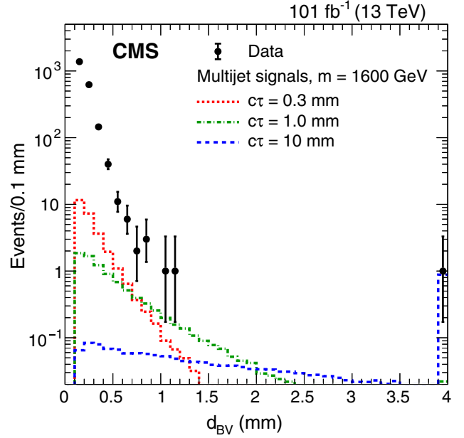
FIG. 5. The distribution of d_{BV} for \geq 5 -track one-vertex events in data and three simulated multijet signal samples each with a mass of 1600 GeV. The production cross section for each signal model is assumed to be the lower limit excluded by Ref. [25], corresponding to values of 0.8, 0.25, and 0.15 fb for the samples with c\tau = 0.3, 1.0 , and 10 mm, respectively. The last bin includes the overflow events. This bin includes one event in data with a vertex with large d_{BV} that appears to arise from tracks originating from separate pp interaction vertices, consistent with background.
