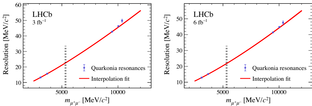
FIG. 5. Fit to the measured mass resolutions of quarkonia resonances (blue dots) with a power-law function to obtain the mass resolution at the B^0 and B_s^0 masses as indicated by the two dashed lines in (left) Run 1 and (right) Run 2 data.
